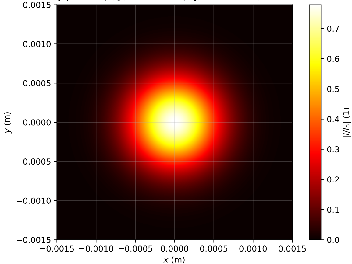
Intensity profile I(x, y, z = 1.194m)/I_0 , \text{Pin}=0.1\text{Pcr} , artificial time
